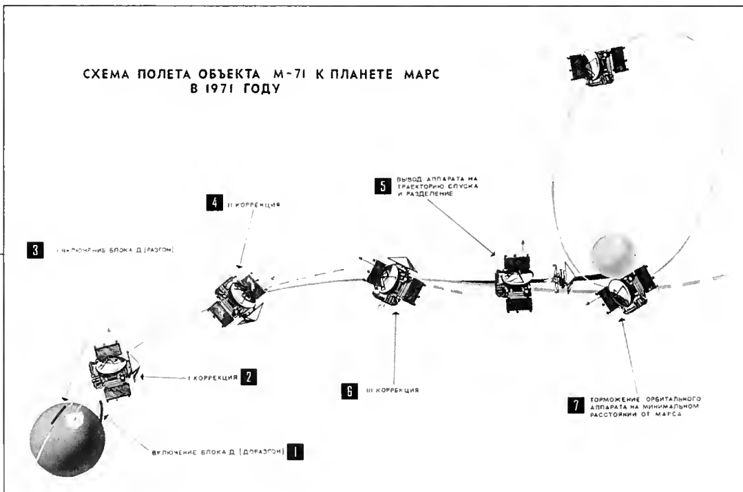
Figure 16. The Flight Profile of the Mars 2 and 3 Spacecraft to Mars in 1971— (1) activation of block D (before boosting), (2) first correction, (3) activation of block D (boosting), (4) second correction, (5) injection of the spacecraft in the descent trajectory and separation, (6) third correction, and (7) braking of the orbiter at the minimal distance from Mars
